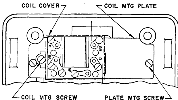
Fig. 1—Induction Coil Mounting
