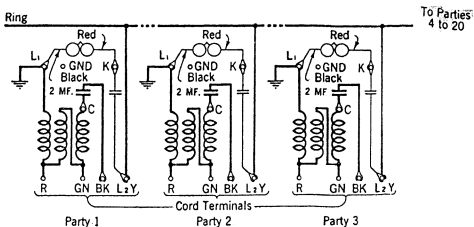
Fig. 3—Grounded Return Line Anti-Sidetone Stations High Impedance Ringers
