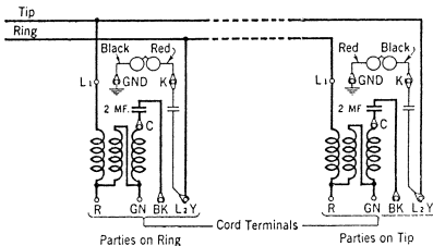
Fig. 2—Divided Code Ringing Anti-Sidetone Stations—High Impedance Ringers
