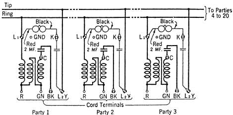
Fig. 1—Bridged Ringing Anti-Sidetone Stations—High Impedance Ringers
