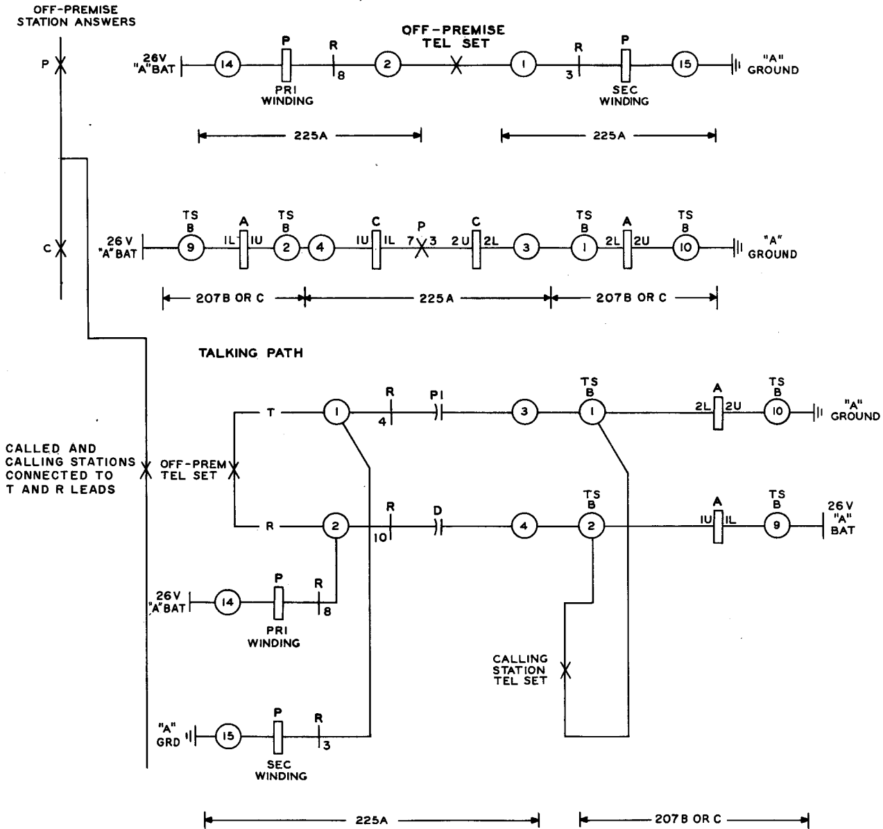
Fig. 11 - Off-Premise Station, Answering Incoming Call
