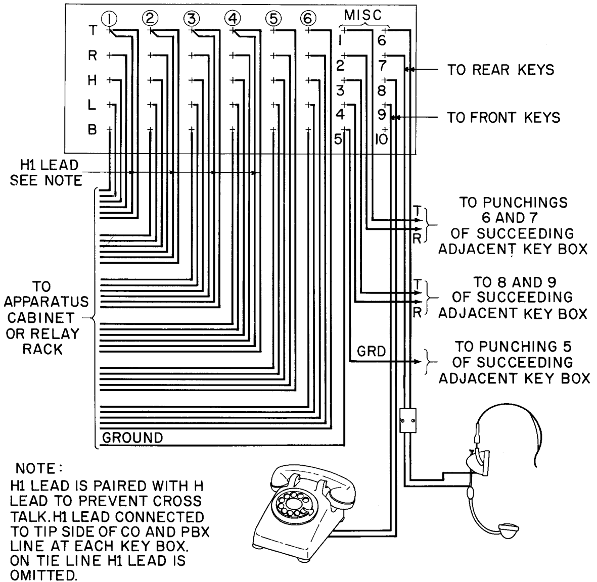
Fig. 1 — 6-line Double-sided Key Box — Terminal Connections
