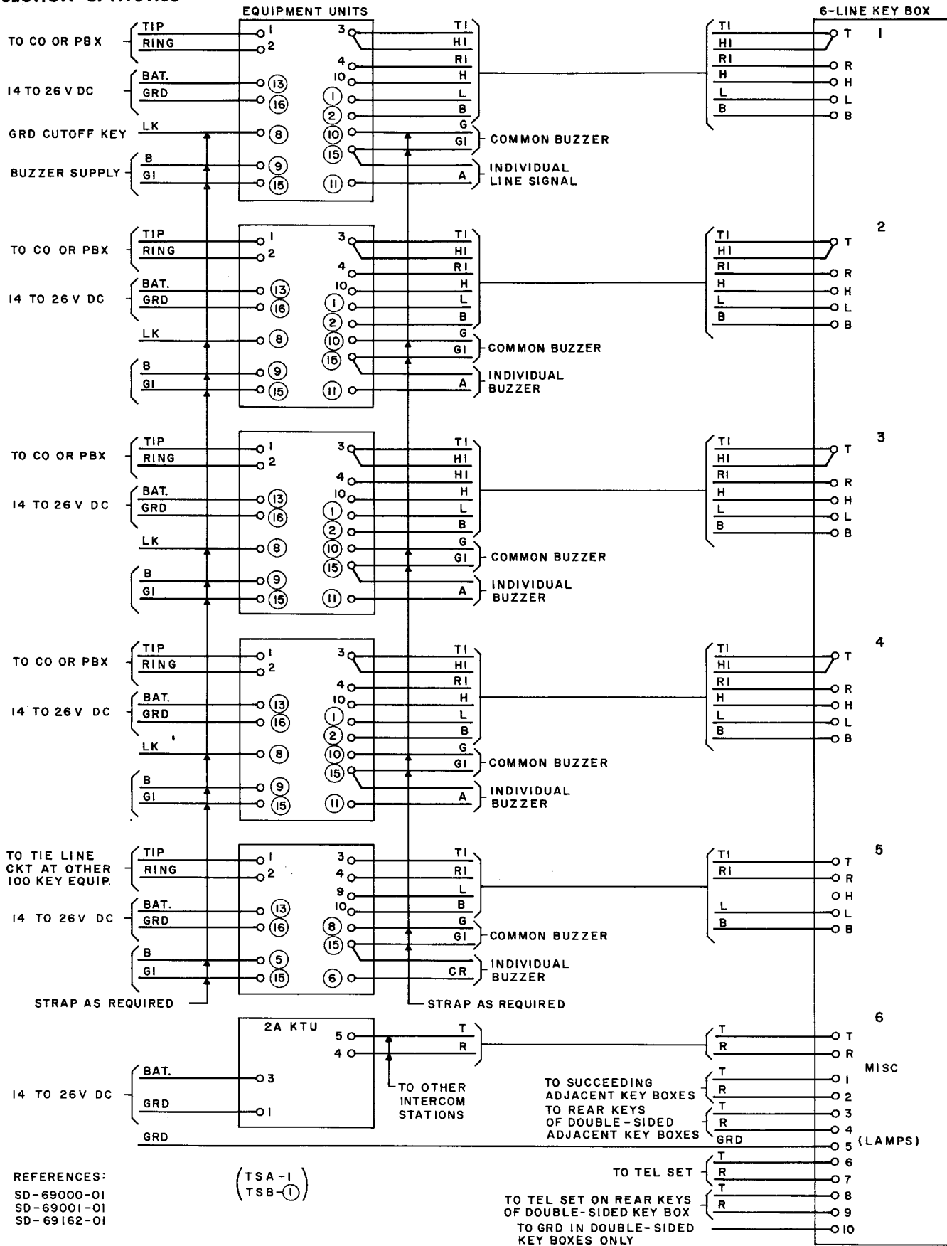
Fig. 2 - 100 Key Equipment Connection Diagram
