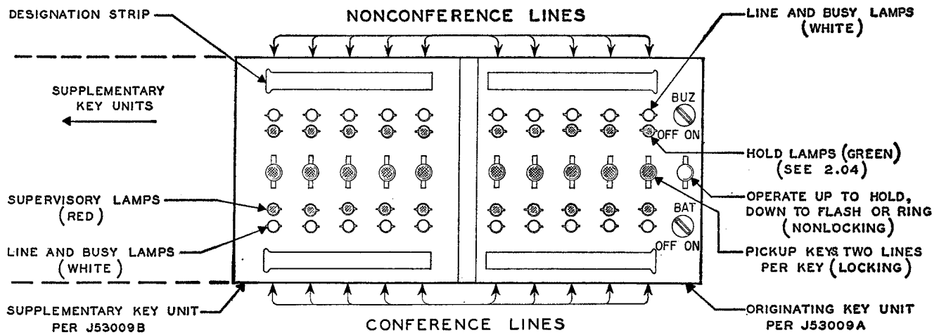
Fig. 1 – Type 1 Position
