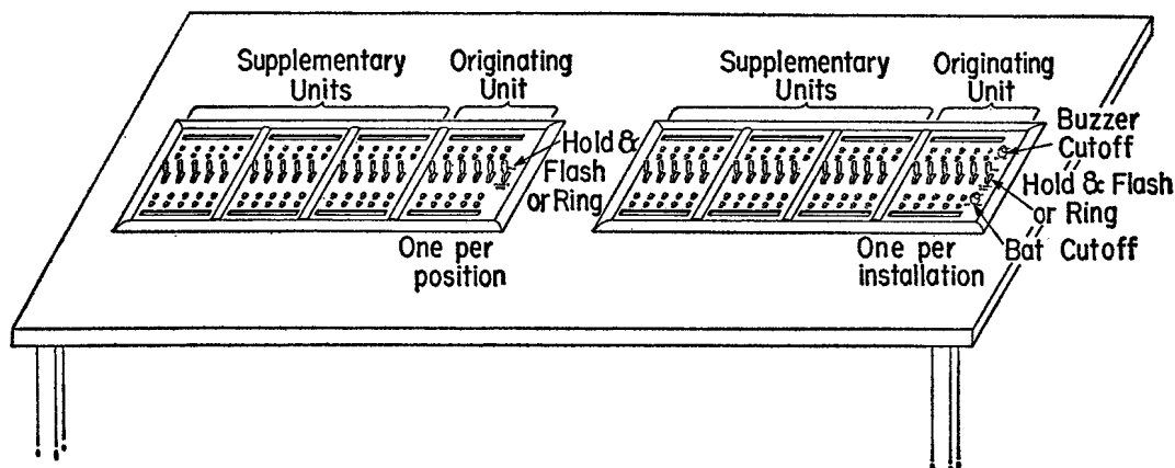
Fig. 4 — Flush-mounting Arrangement
