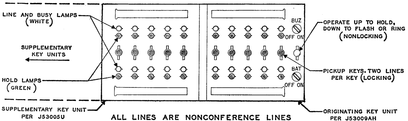
Fig. 2 – Type 2 Position
