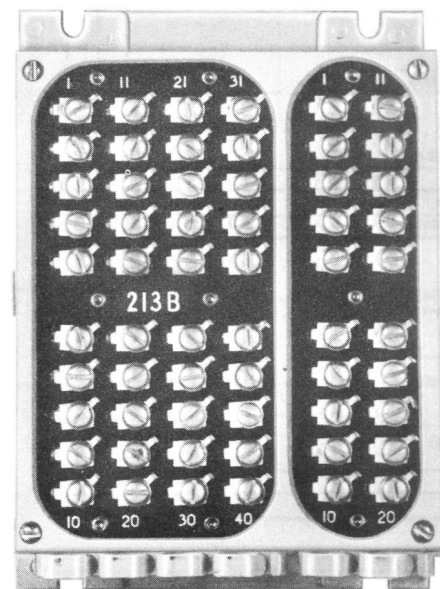
Fig. 2 - 213B KTU, Rear View
