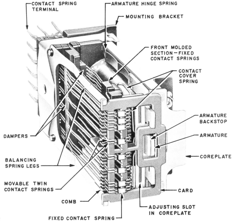
Fig. 1 - Typical Wire-Spring Relay, Without Cover
